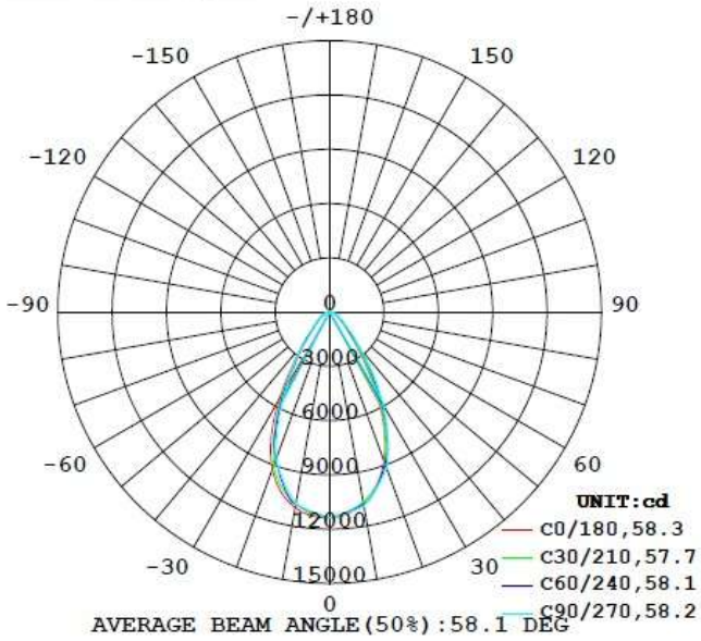
100W-Beam Angle 60°
